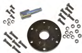
3 1/8 in Flanged To 1 5/8 in EIA Flanged 50 Ohm 4600-025
